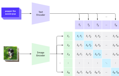
1. Contrastive pre-training
