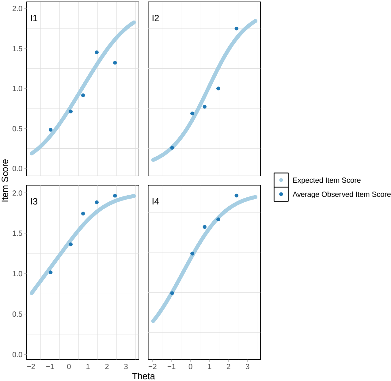
Conditional Item Characteristic Curves
