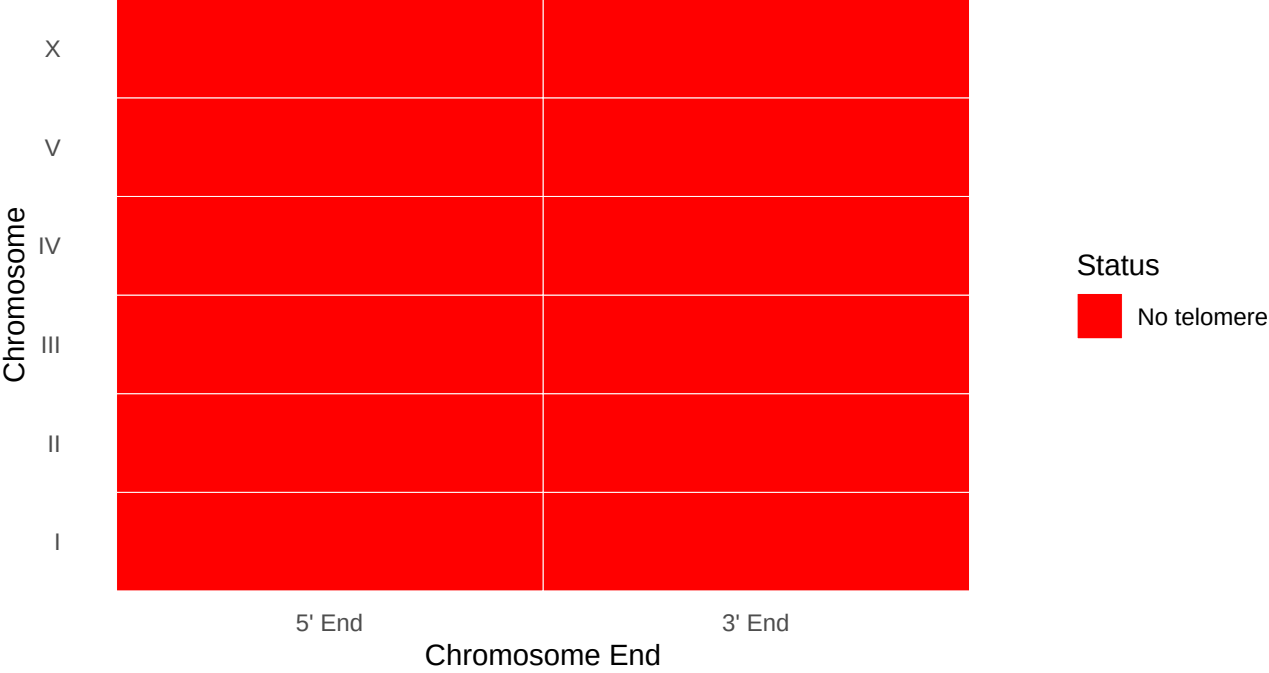
Telomere Status for Oscheius sp. DF5120
