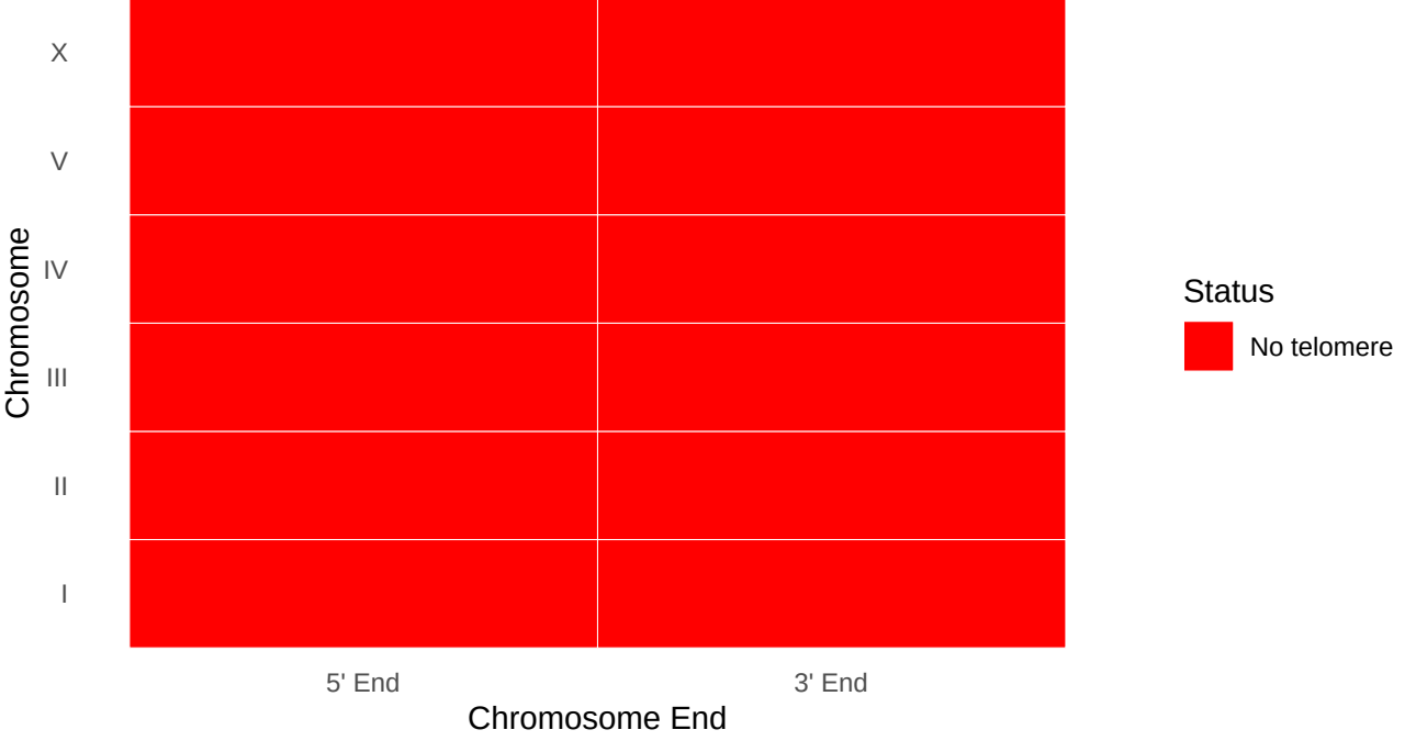
Telomere Status for Oscheius sp. JU1382
