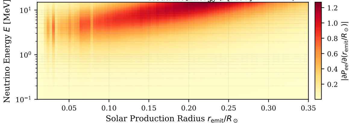
(c) Functional core sensitivity map |\partial P_{ee}/\partial (r_{\text{emit}}/R_{\odot})| across solar interior
