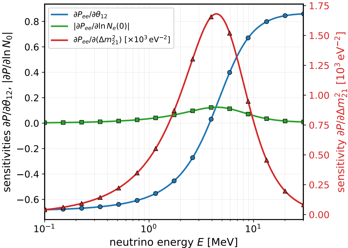
(a) solar parameter sensitivities &amp; FD benchmark
