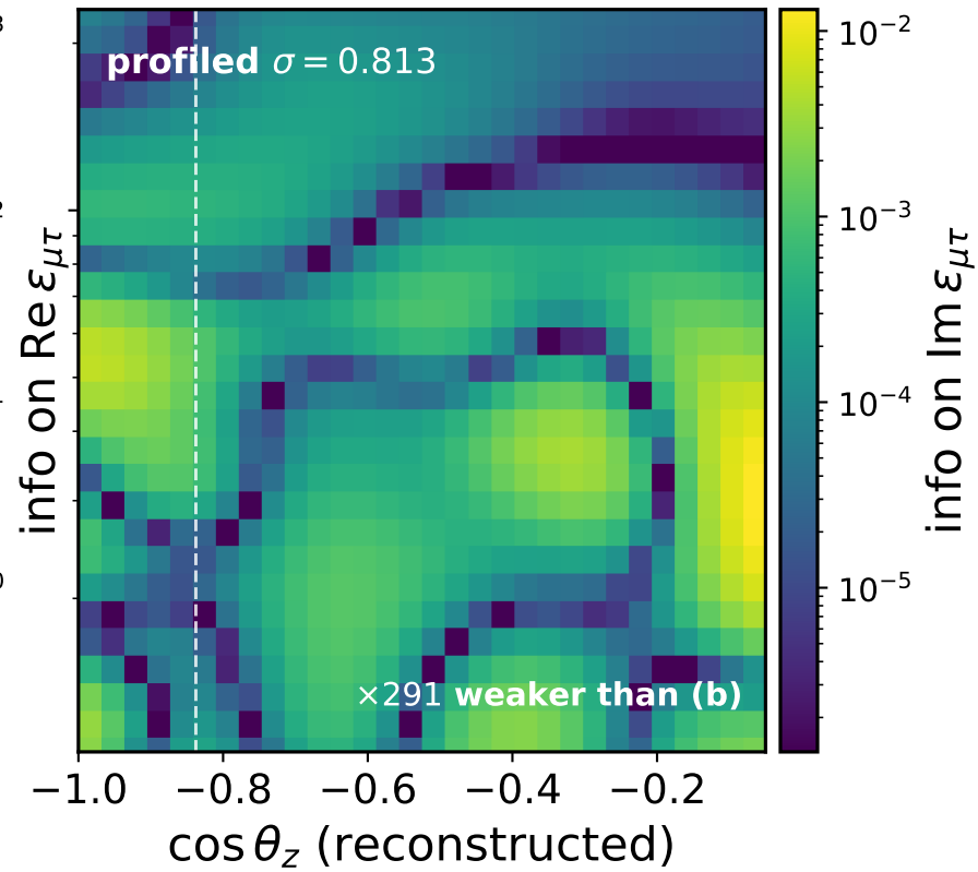
(c) profiled info: \text{Im } \epsilon_{\mu\tau}
