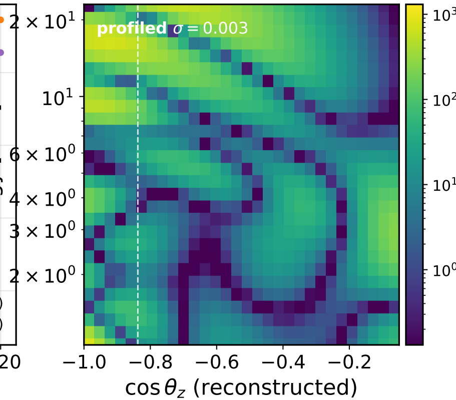
(b) profiled info: \text{Re } \epsilon_{\mu\tau}
