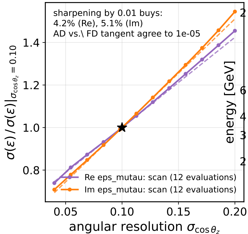
(a) NSI bound vs. detector resolution
