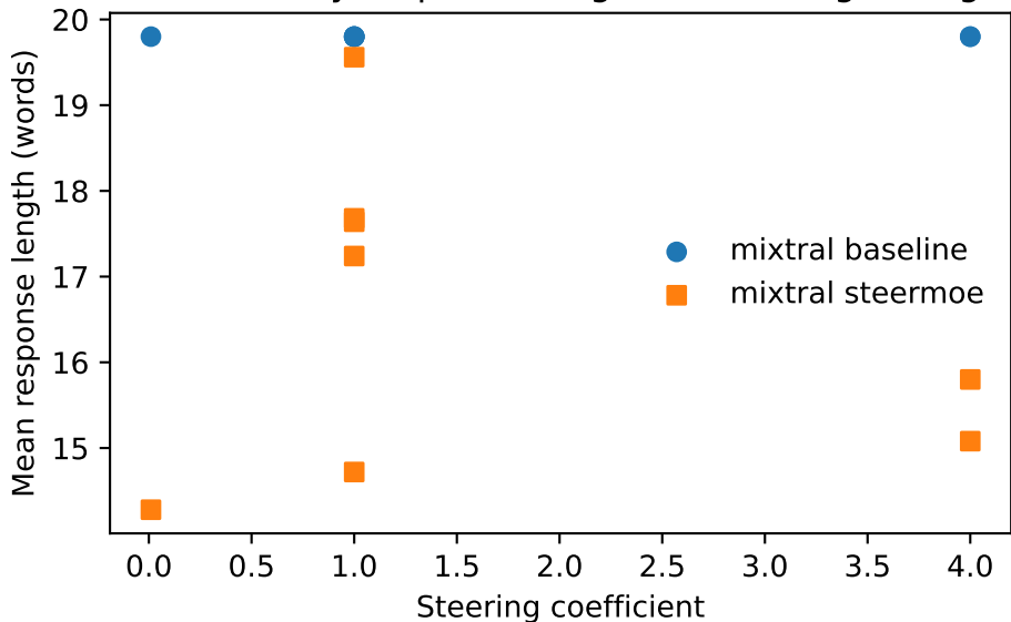
Question-only response length vs steering strength
