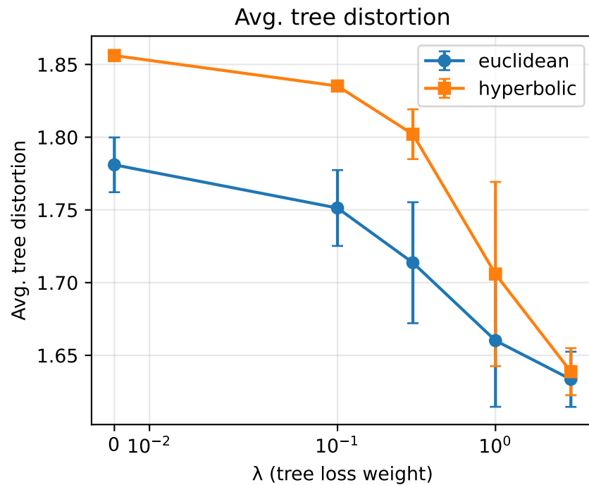
Hierarchy-aware loss at d=8 , c=1.0
