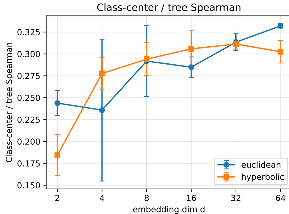
Scaling with d (hyperbolic = best curvature per d)
