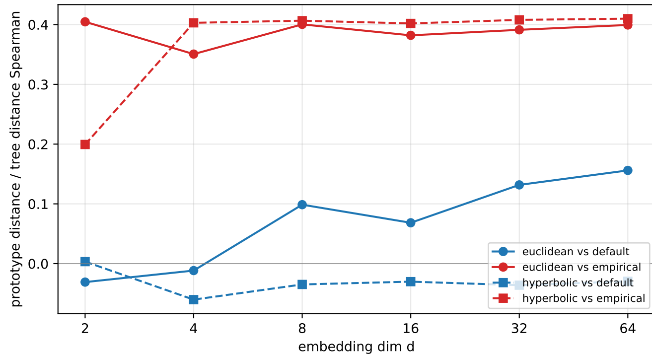
Prototype distances vs reference tree
