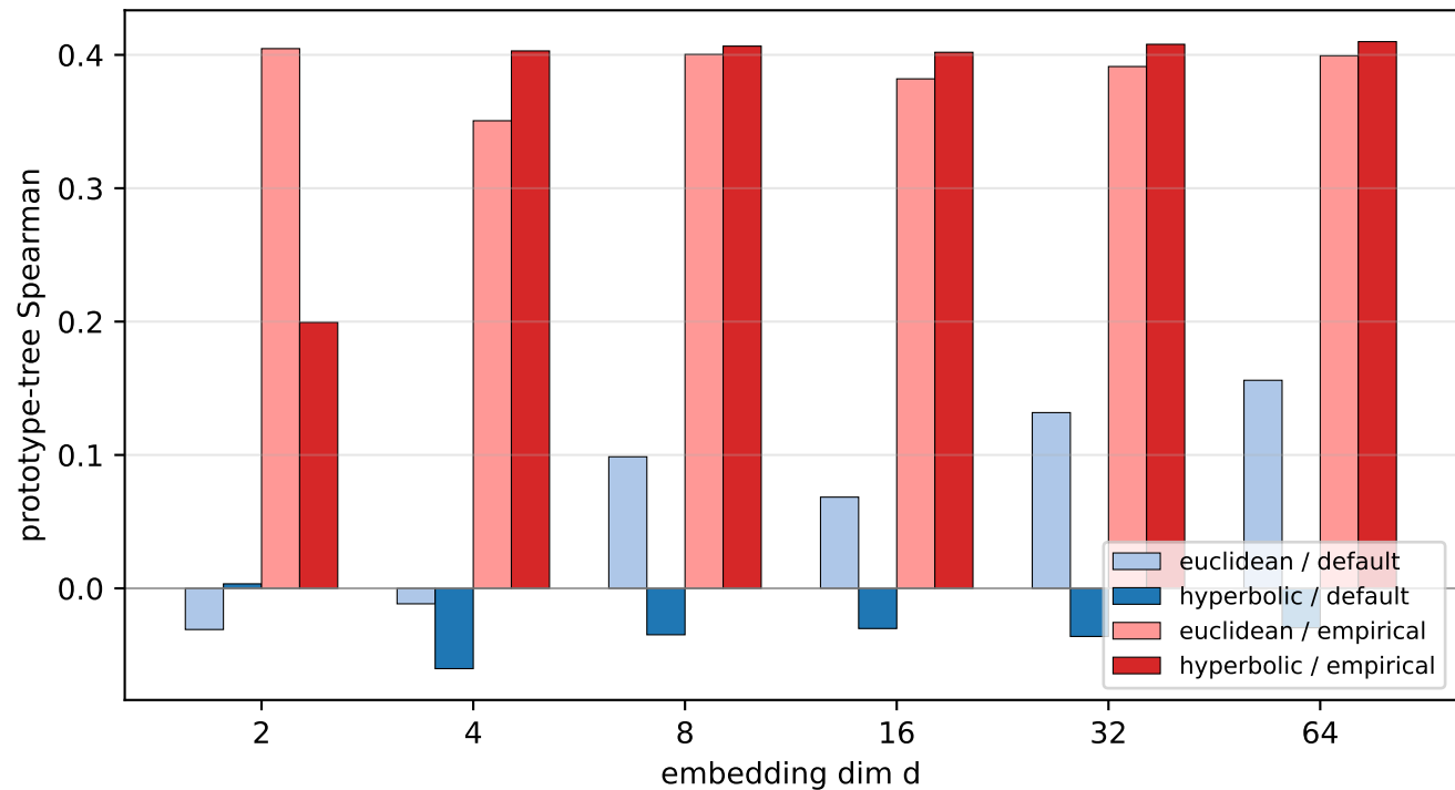
Geometry winner depends on the choice of reference tree
