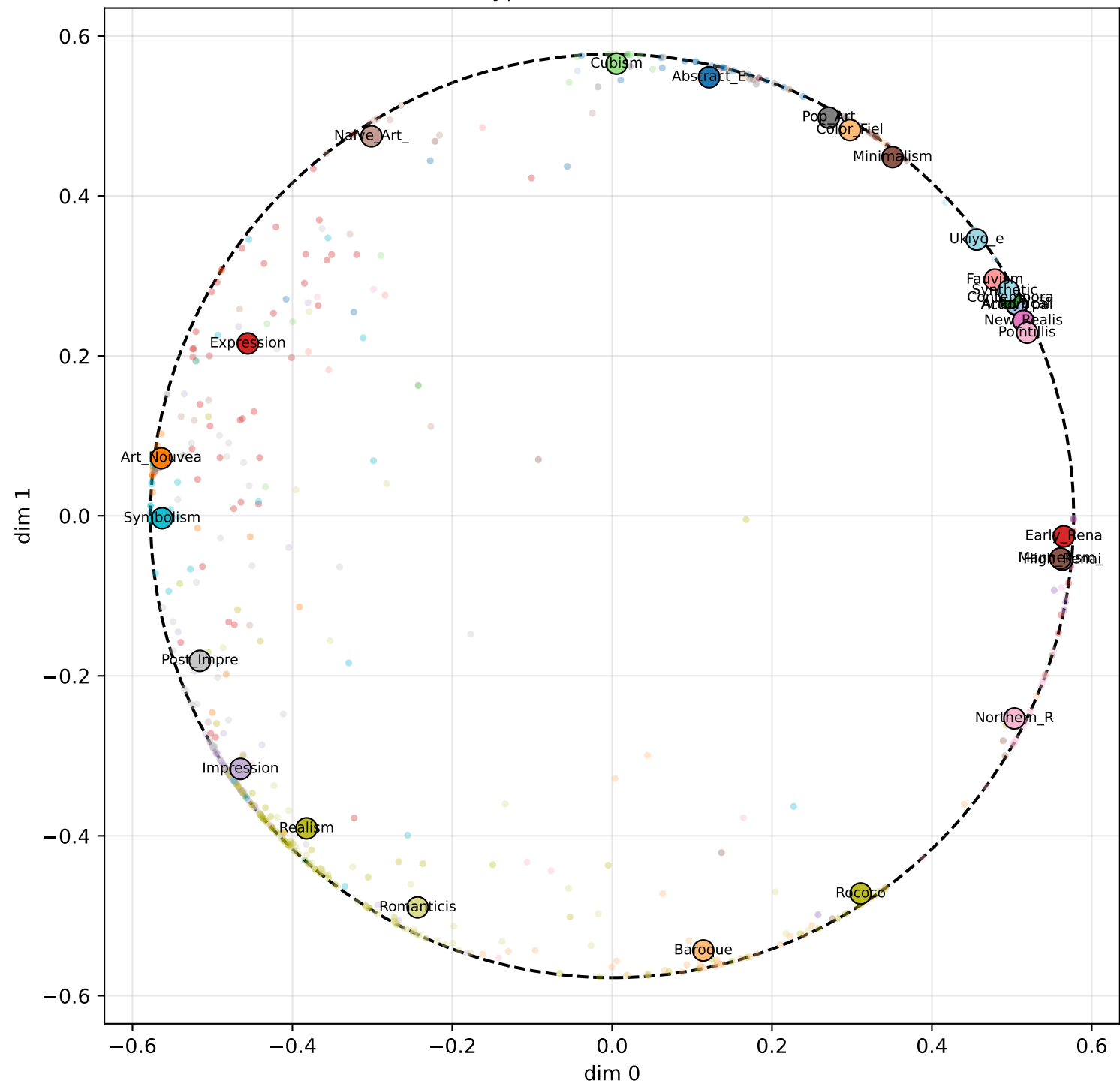
hyperbolic d=2, c=3.0
