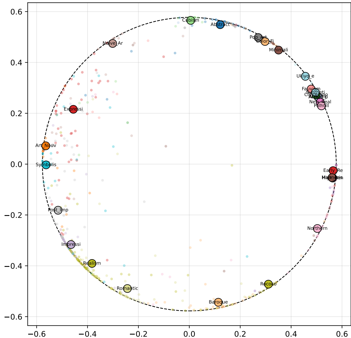
hyperbolic d=2, c=3.0
