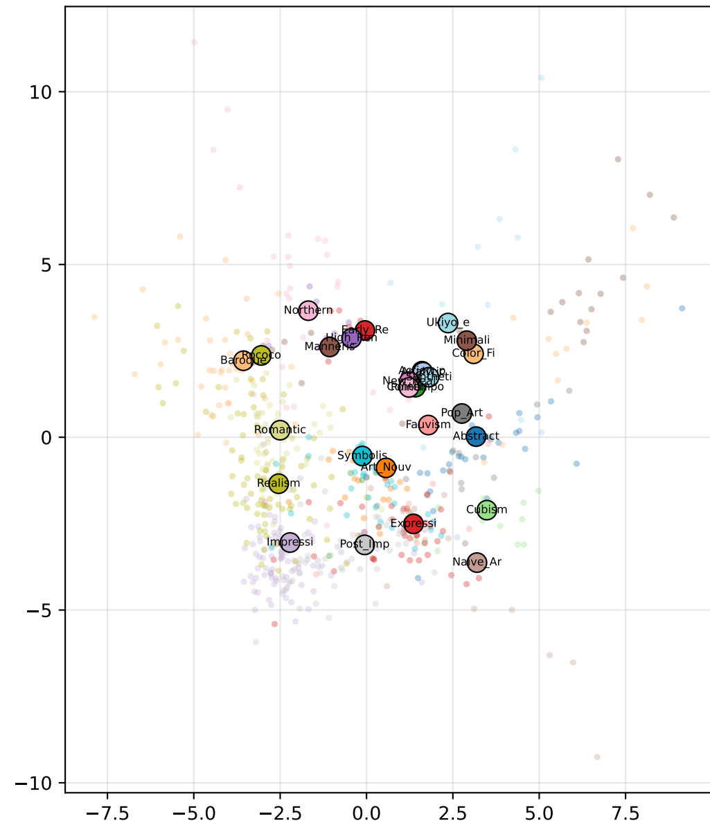
euclidean d=2
