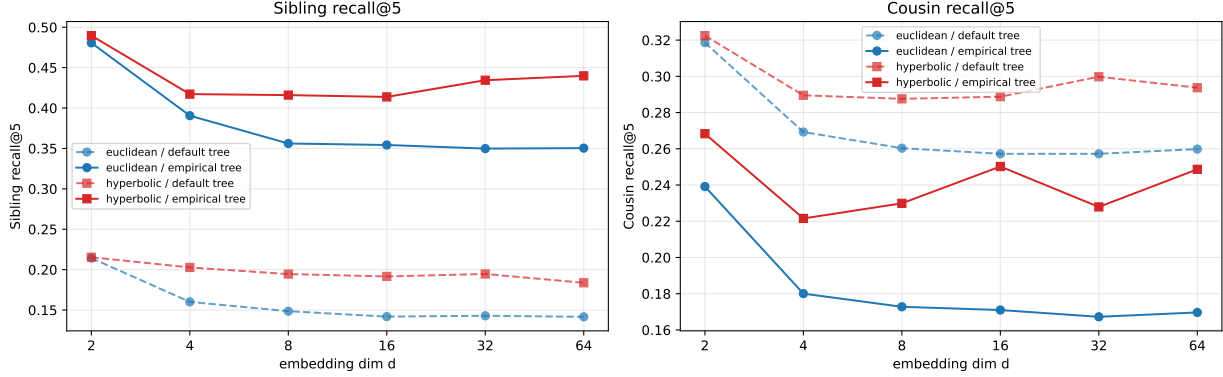
Figure 3. Sibling and cousin recall@5 with relations defined by the default tree (dashed) and a CLIP-derived empirical tree (solid), per geometry per embedding dimension. The hyperbolic lead is preserved under the empirical-tree redefinition; on sibling recall the gap widens slightly. The DINOv2-derived empirical tree is in Section F.
