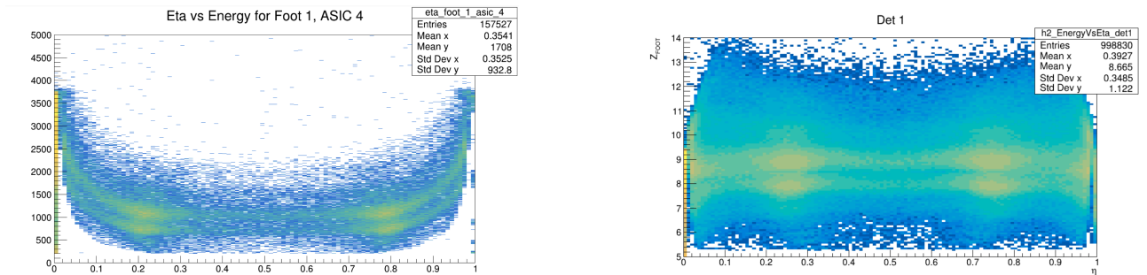
Figure 1: Energy as a function of the eta parameter. Left: With eta correction or charge calibration, only one ASIC. Right: After eta correction and charge calibration for all the ASICs of the detector.
