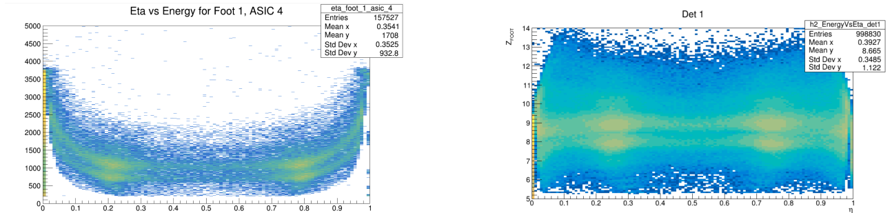
Figura 1: Energy as a function of the eta parameter. Left: With eta correction or charge calibration, only one ASIC. Right: After eta correction and charge calibration for all the ASICs of the detector.
