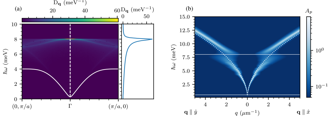
FIG. 4. Coupling between plasmons and the magnon continuum in a quasi two-dimensional antiferromagnet [Fig. 1c]. (a) Magnon dispersion in the k_x - k_y plane, with the white line indicating \epsilon_k . The dashed white line indicates the steep plasmon dispersion and the colorscale is the spin-zero two-magnon density of states. Shown on the right is a cut of the spin-zero two-magnon density of states along the plasmon energy. (b) The plasmon spectral function A_q(\epsilon) along two propagation directions of the plasmon: \mathbf{q} \parallel \hat{x} and \mathbf{q} \parallel \hat{y} [see Fig. 1(a) for real space geometry]. The lower and upper edges of the spin-zero two-magnon continuum are indicated by the horizontal white lines. The bare plasmon dispersion is indicated by the white dotted line. We stress that the plasmon spectral function is shown on a logarithmic scale.
