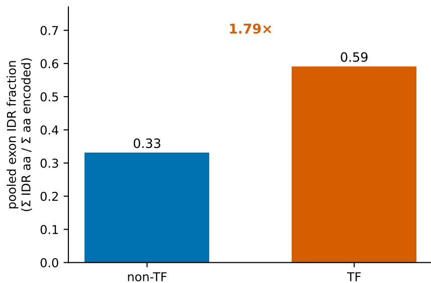
B Pooled exon IDR fraction
