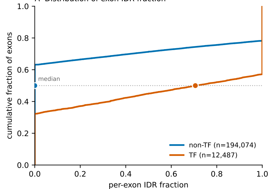
A Distribution of exon IDR fraction
