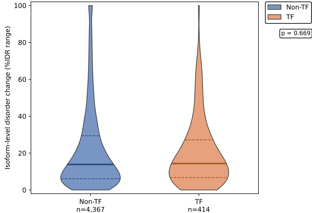
TFs vs. Non-TFs Isoform-Level Disorder Variation Among IDR-Containing Genes
