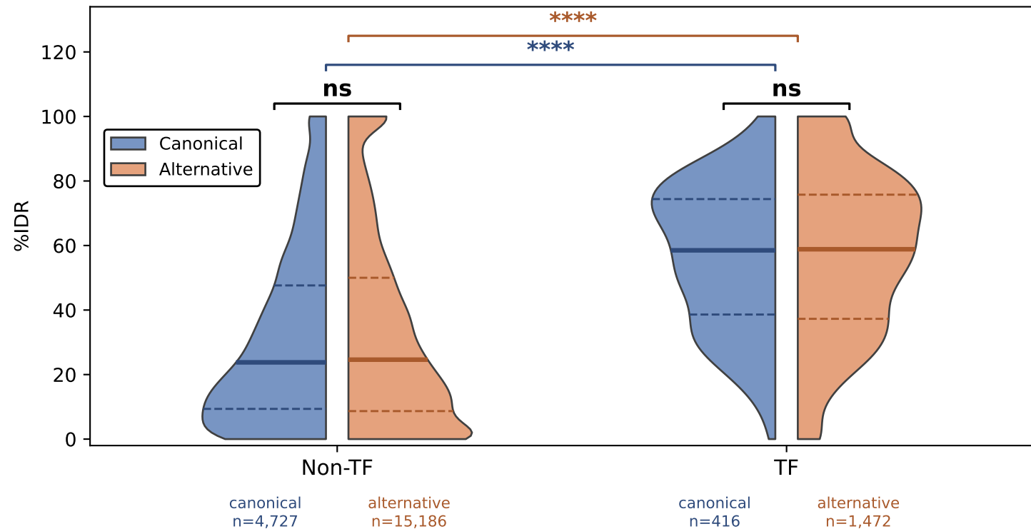
TFs vs. Non-TFs Isoform Disorder Content (canonical vs alternative)
