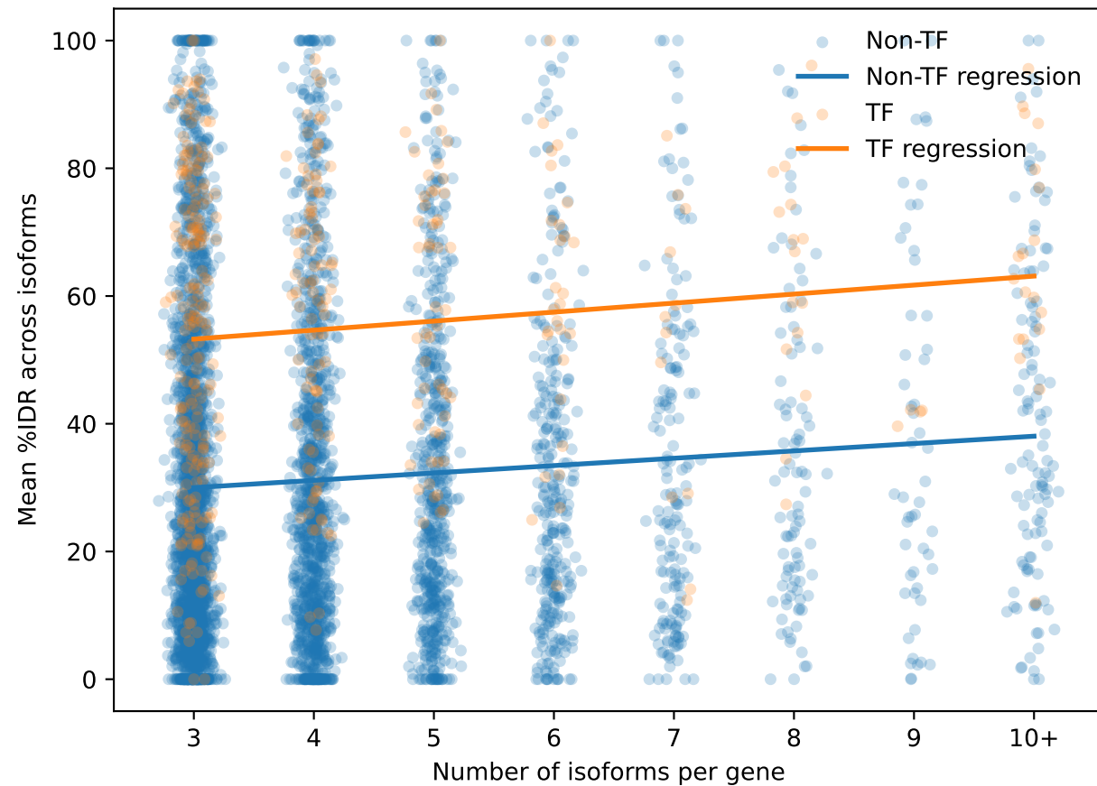
Number of isoforms vs mean %IDR
