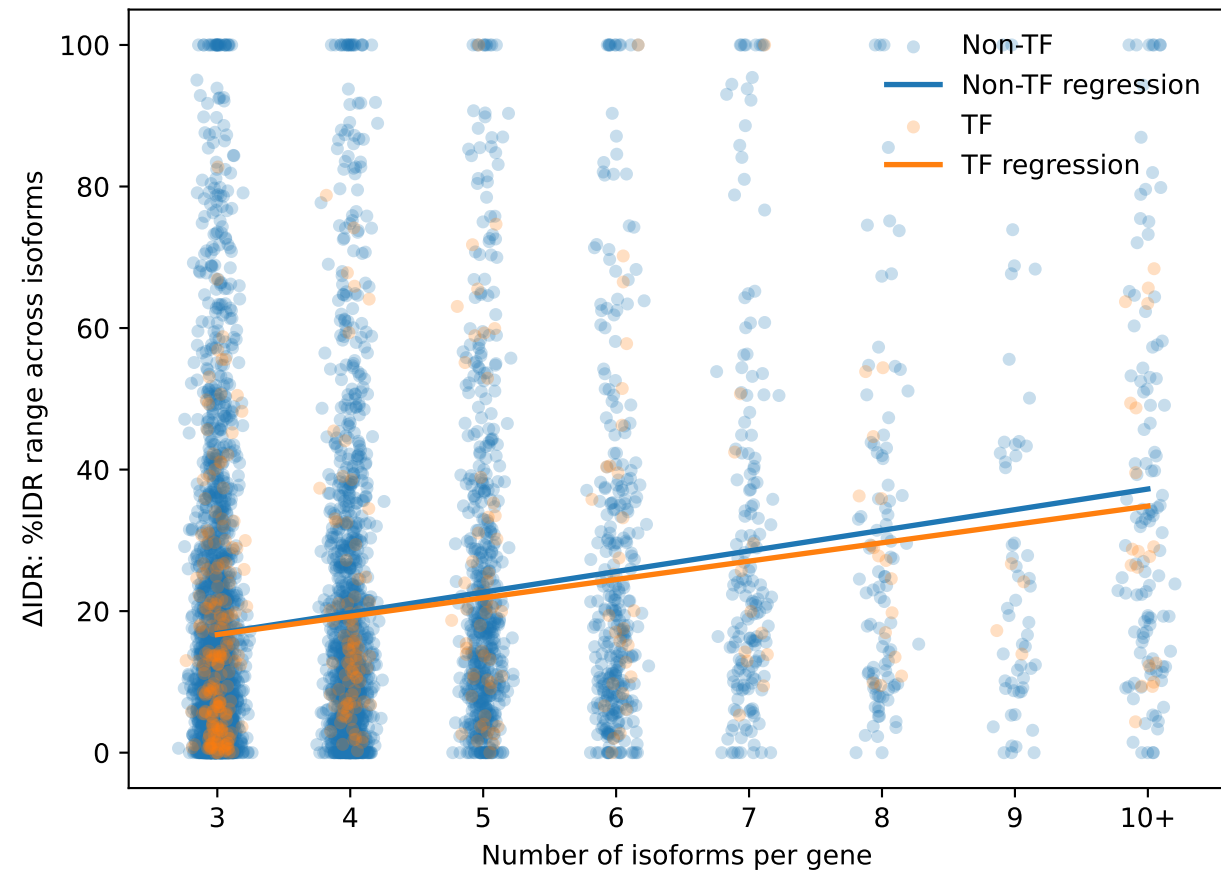
Number of isoforms vs isoform-level \Delta %IDR
