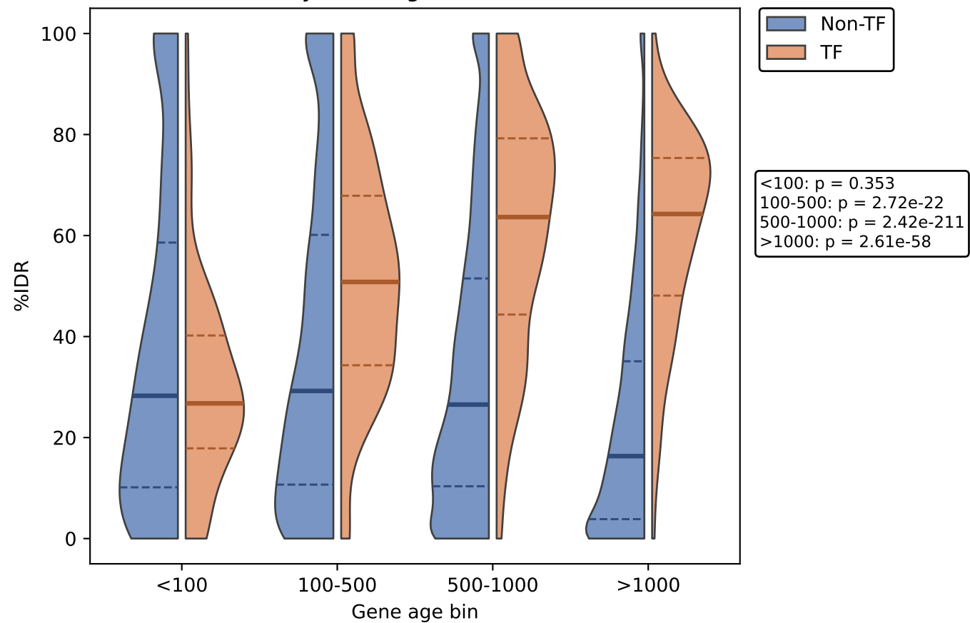
% IDR by Gene Age: TFs vs Non-TFs
