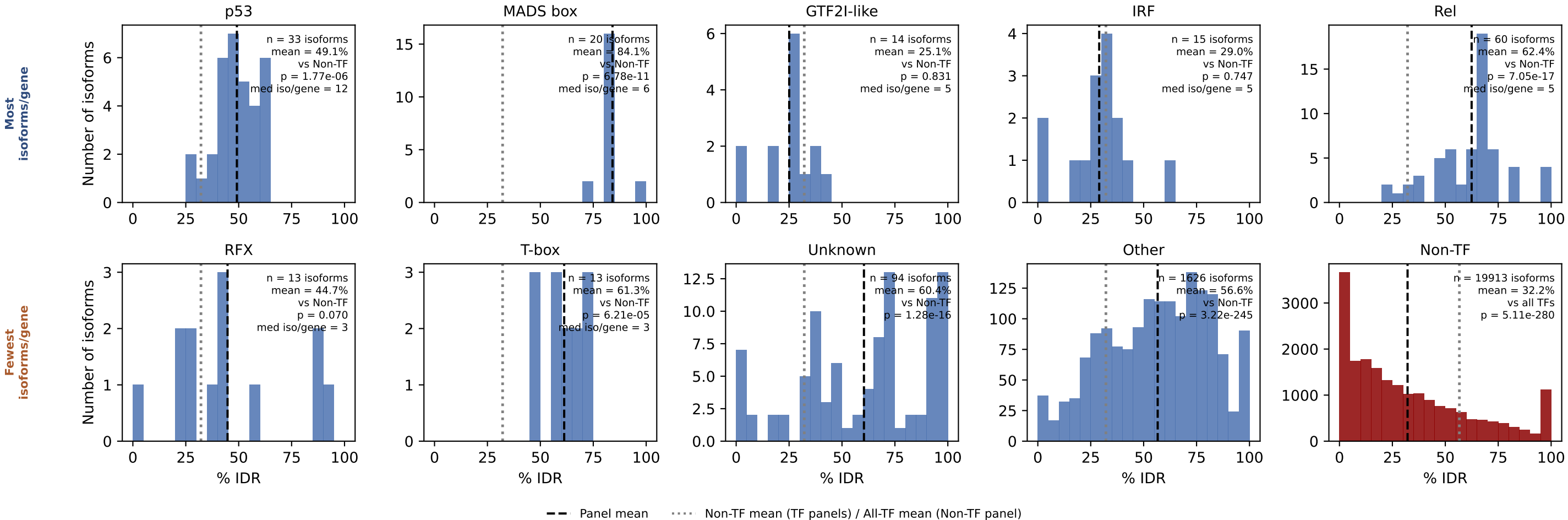
% Disorder per isoform: TF families ranked by isoform count per gene Top row = most isoforms/gene | Bottom row = fewest isoforms/gene + Unknown / Other / Non-TF
