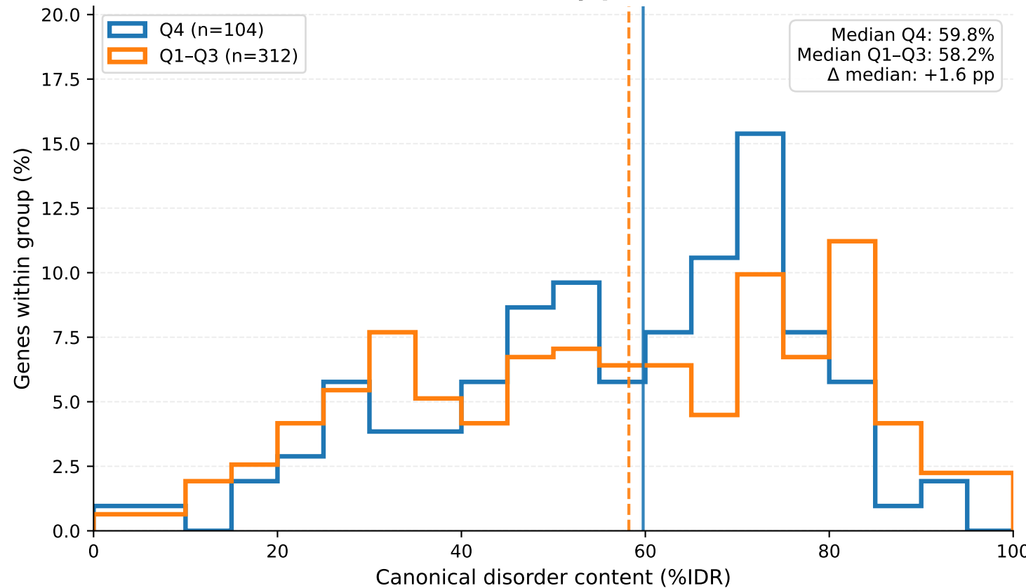
A. Transcription factors Mann-Whitney p = 0.88
