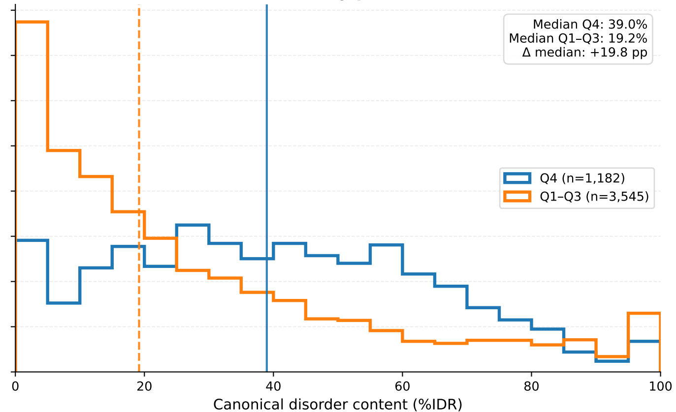
B. Non-transcription factors Mann-Whitney p = 7.3e-62
