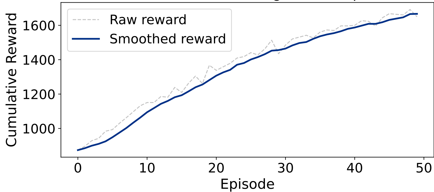
MADRL+GAT Training — antwerp
