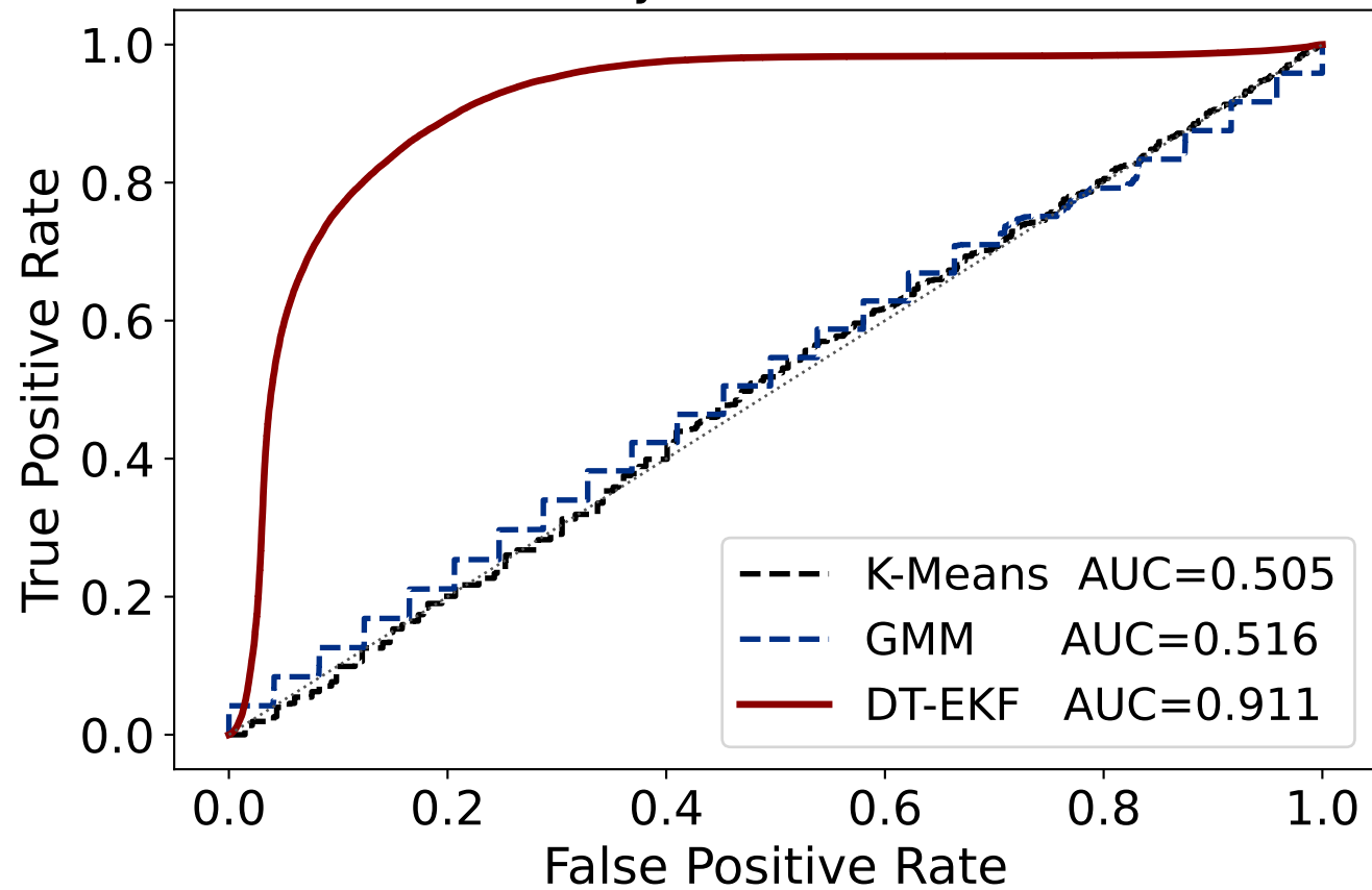
Quality ROC — lorawan
