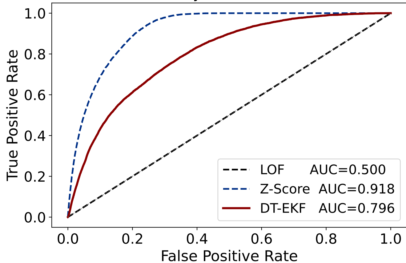
Anomaly ROC — lorawan
