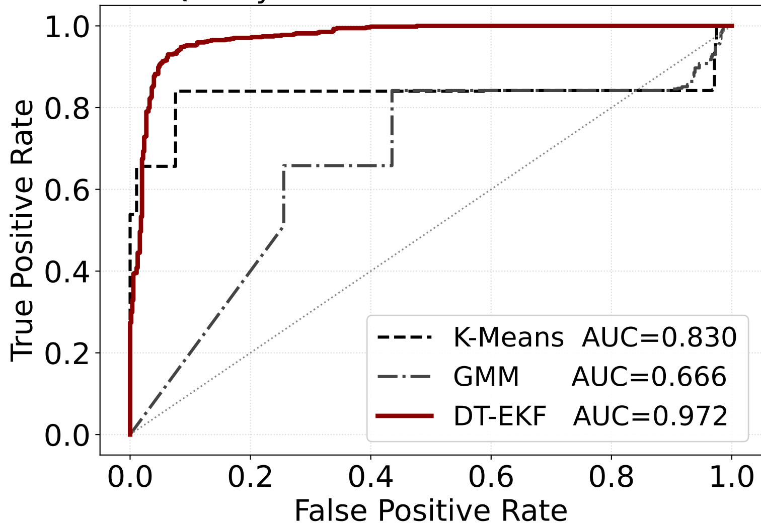
Quality Classification ROC — indoor
