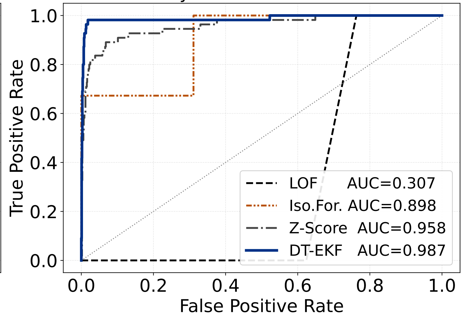
Anomaly Detection ROC — indoor
