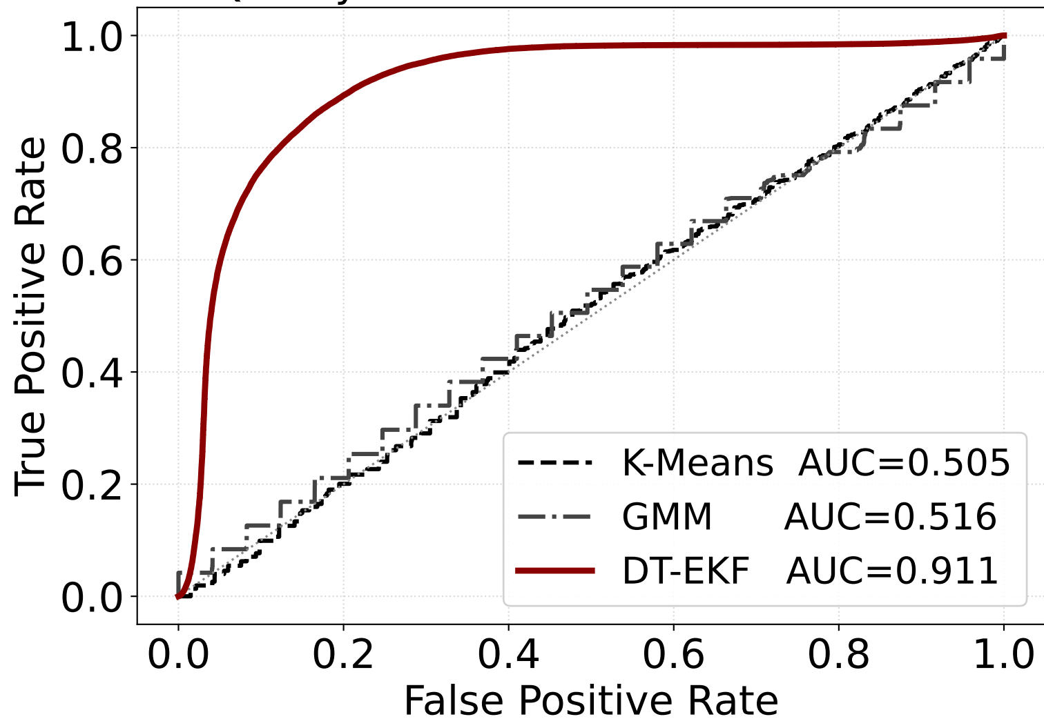
Quality Classification ROC — lorawan
