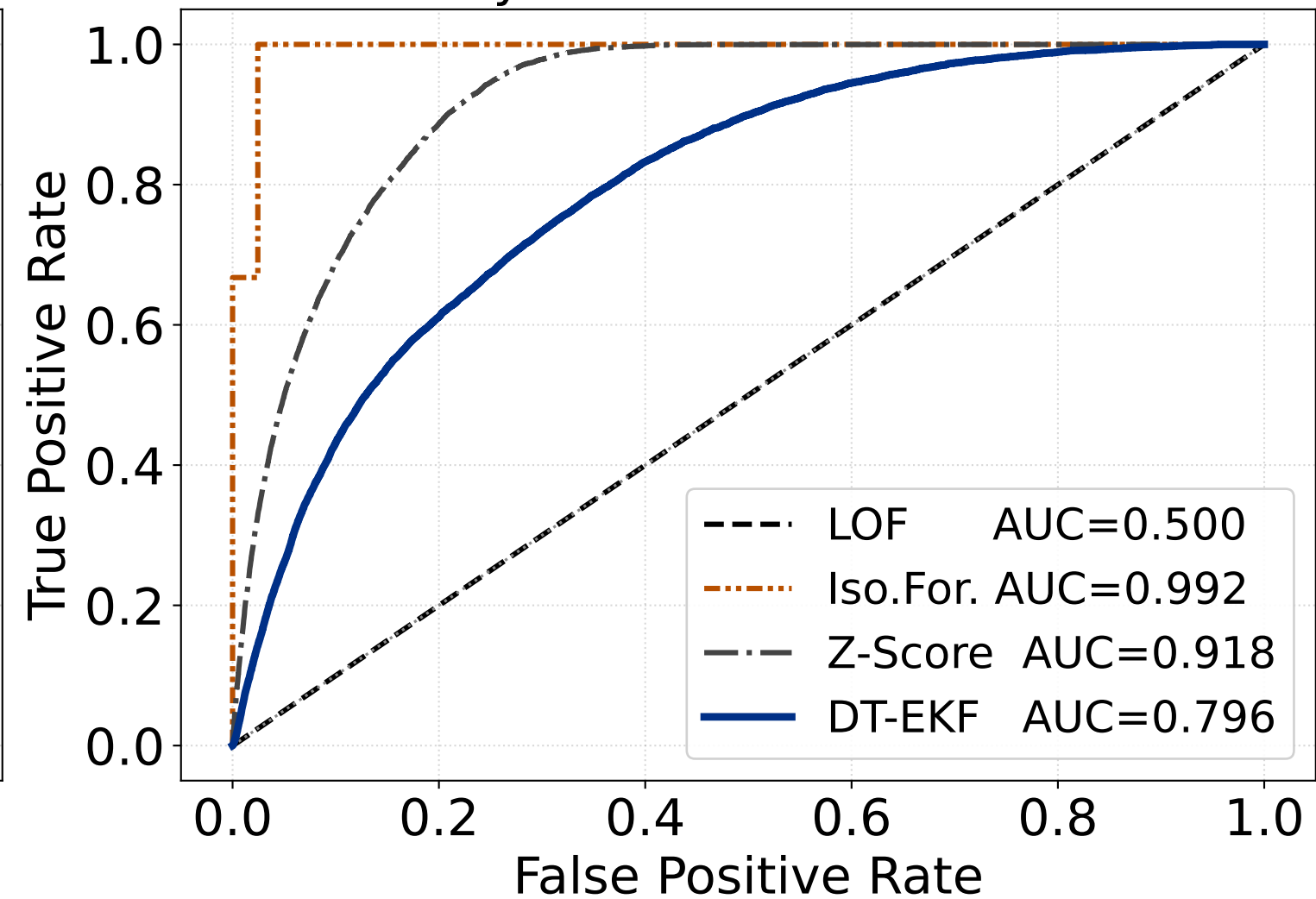
Anomaly Detection ROC — lorawan
