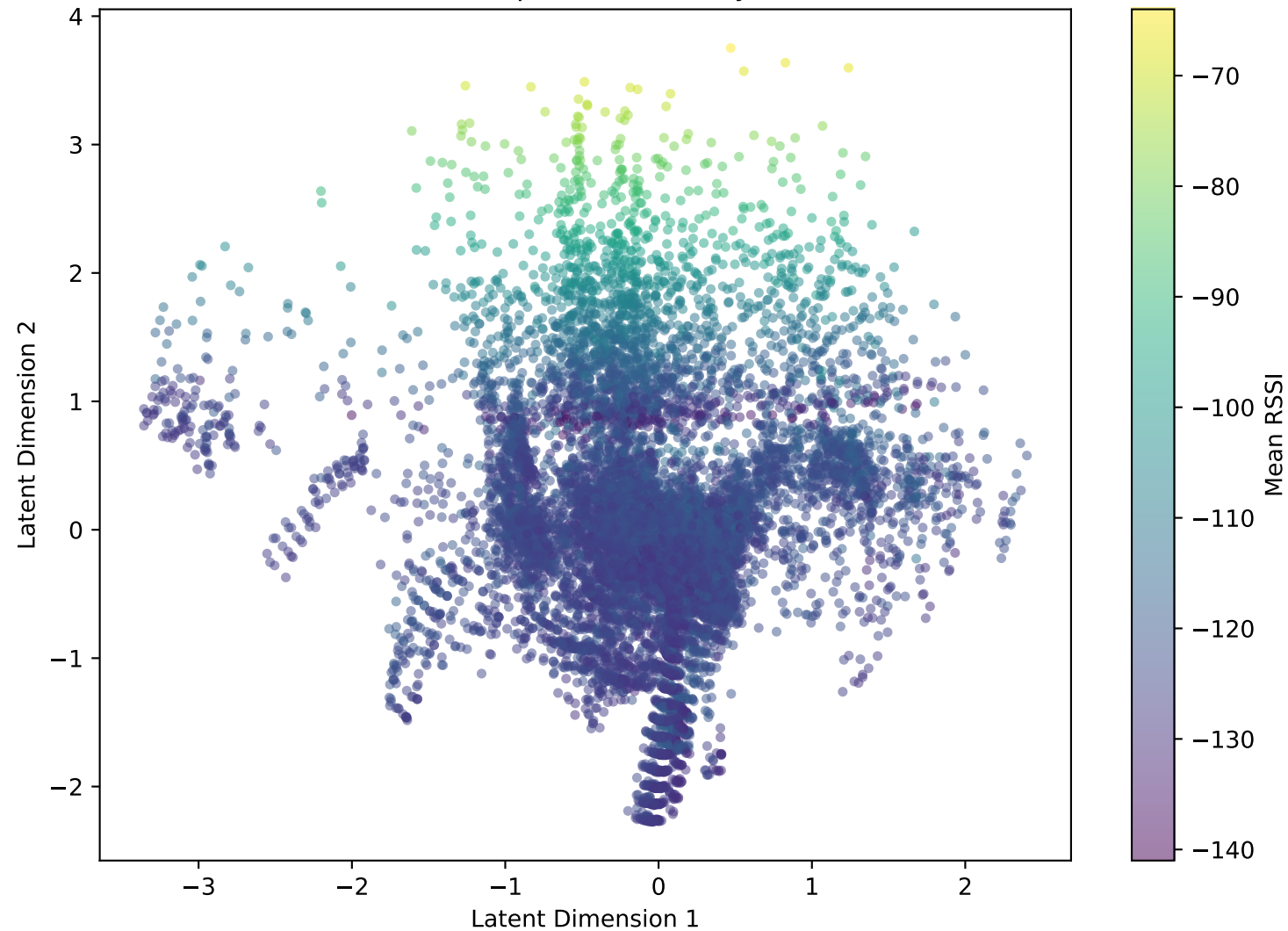
VAE Latent Space (colored by RSSI)
