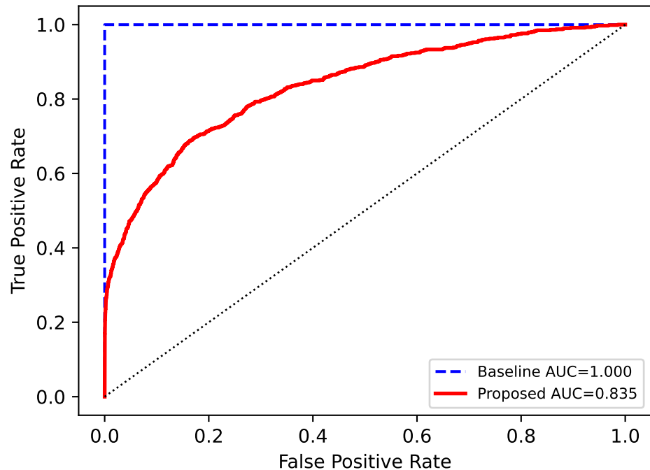
Anomaly Detection ROC — antwerp
