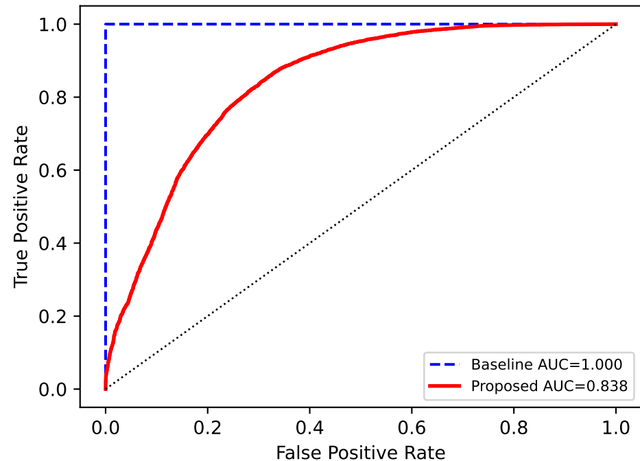
Quality Classification ROC — antwerp
