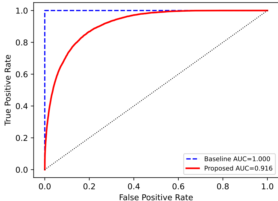
Anomaly Detection ROC — lorawan
