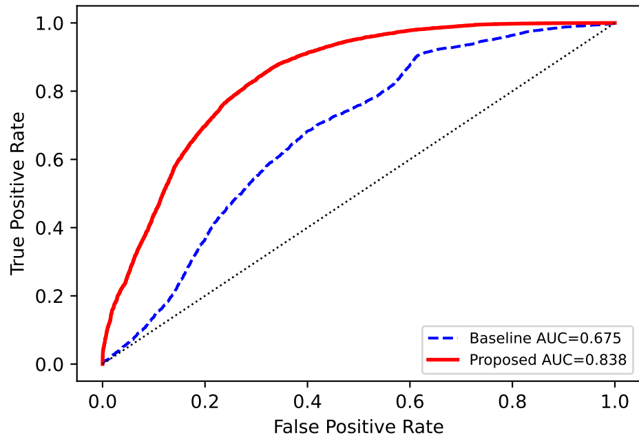
Quality ROC — antwerp (K-Means vs DT-EKF)
