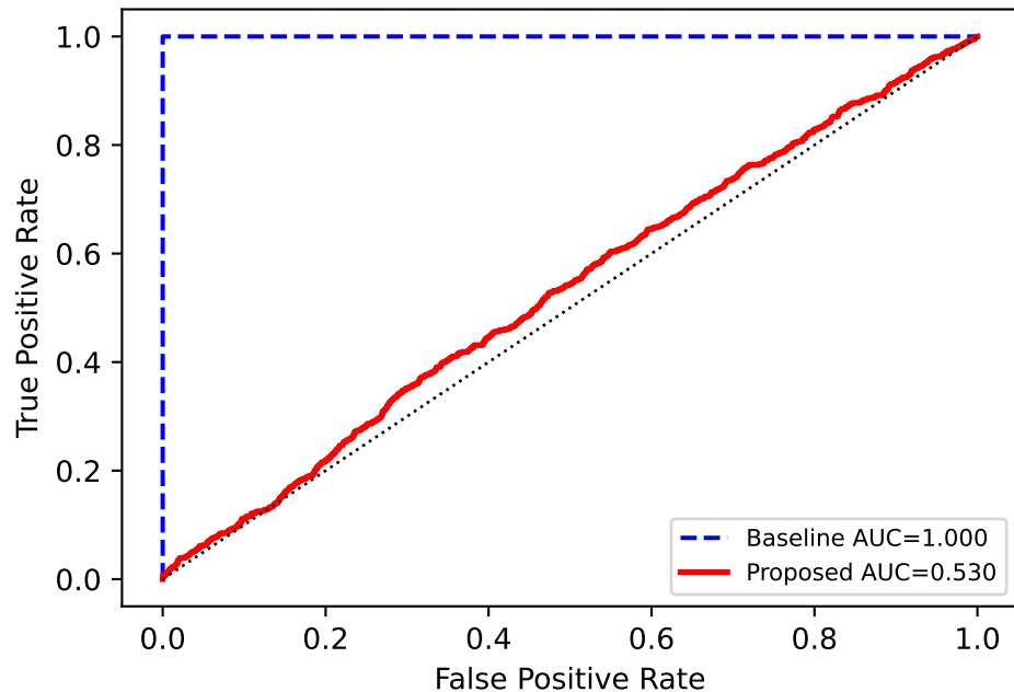
Anomaly ROC — antwerp (LOF vs DT-EKF)
