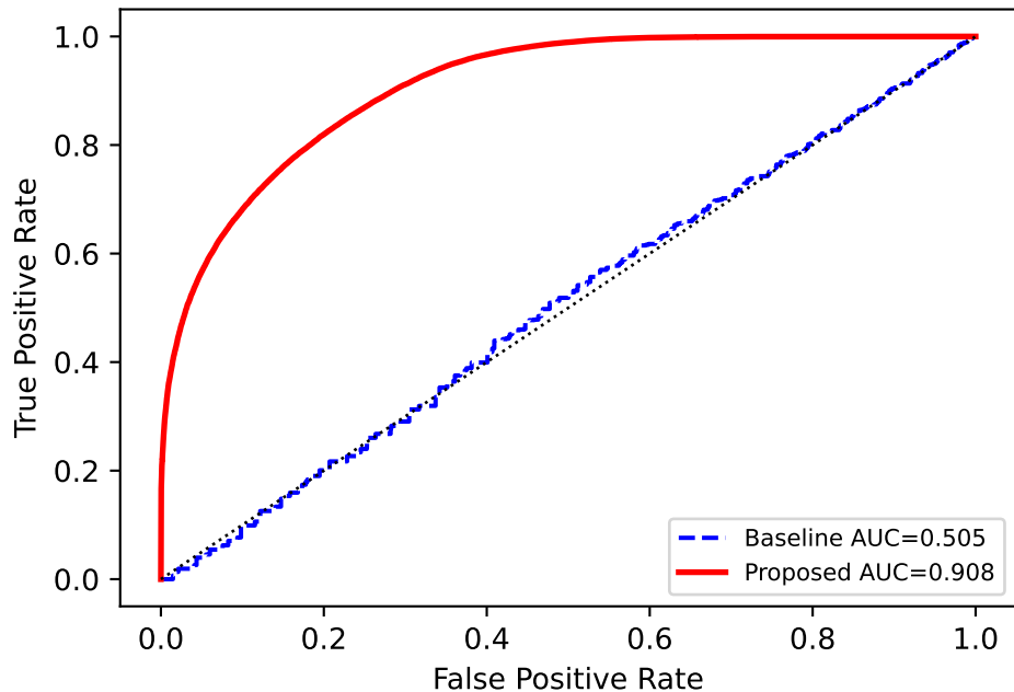
Quality ROC — lorawan (K-Means vs DT-EKF)
