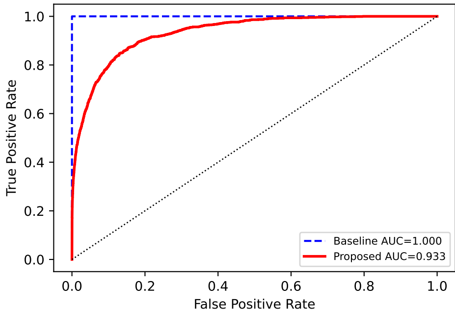
Anomaly ROC — lorawan (LOF vs DT-EKF)
