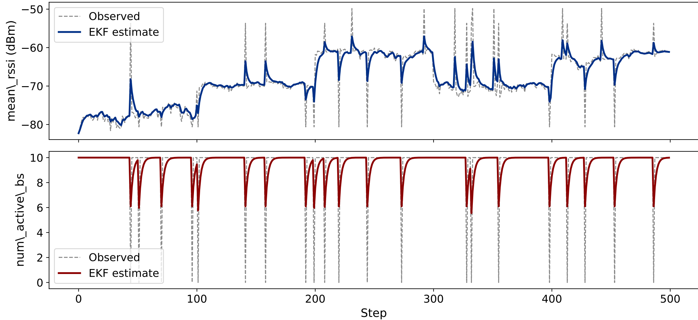
Digital Twin State Estimation — indoor
