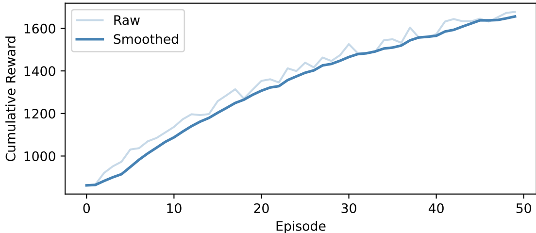
MADRL+GAT Training — antwerp
