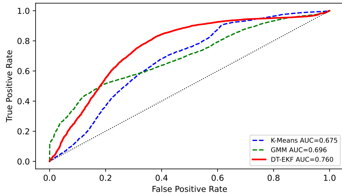
Quality ROC — antwerp (K-Means / GMM vs DT-EKF)
