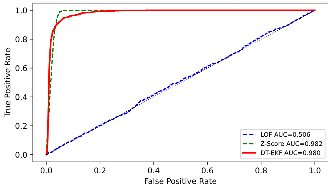
Anomaly ROC — antwerp (LOF / Z-Score vs DT-EKF, fault-injection GT)
