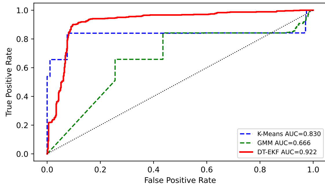
Quality ROC — indoor (K-Means / GMM vs DT-EKF)
