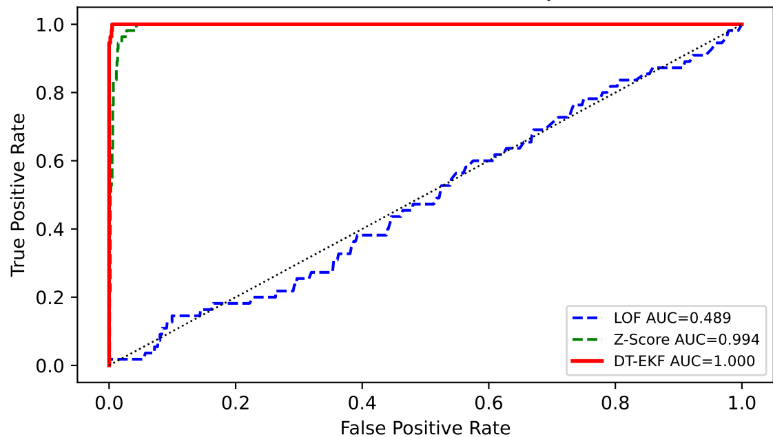
Anomaly ROC — indoor (LOF / Z-Score vs DT-EKF, fault-injection GT)
