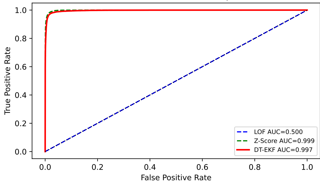
Anomaly ROC — lorawan (LOF / Z-Score vs DT-EKF, fault-injection GT)
