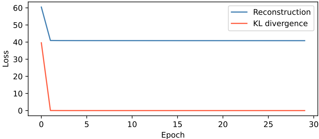
VAE Training Loss — lorawan
