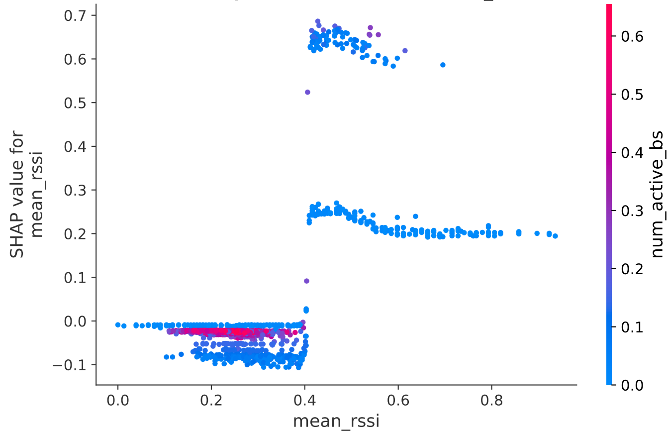
SHAP Dependence Plot for mean_rssi
