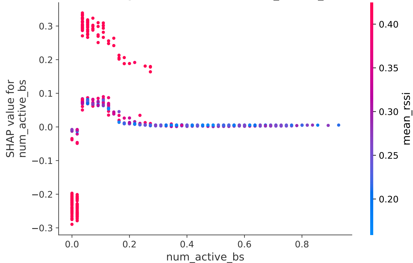
SHAP Dependence Plot for num_active_bs
