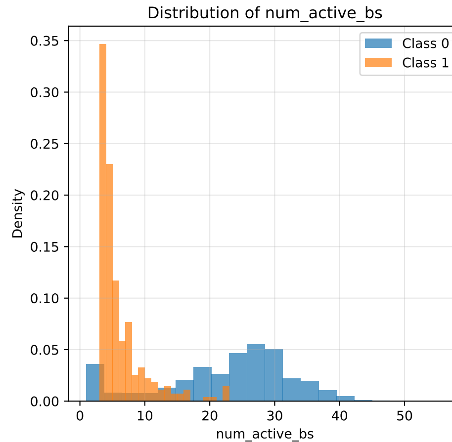
Feature Distributions by Class
