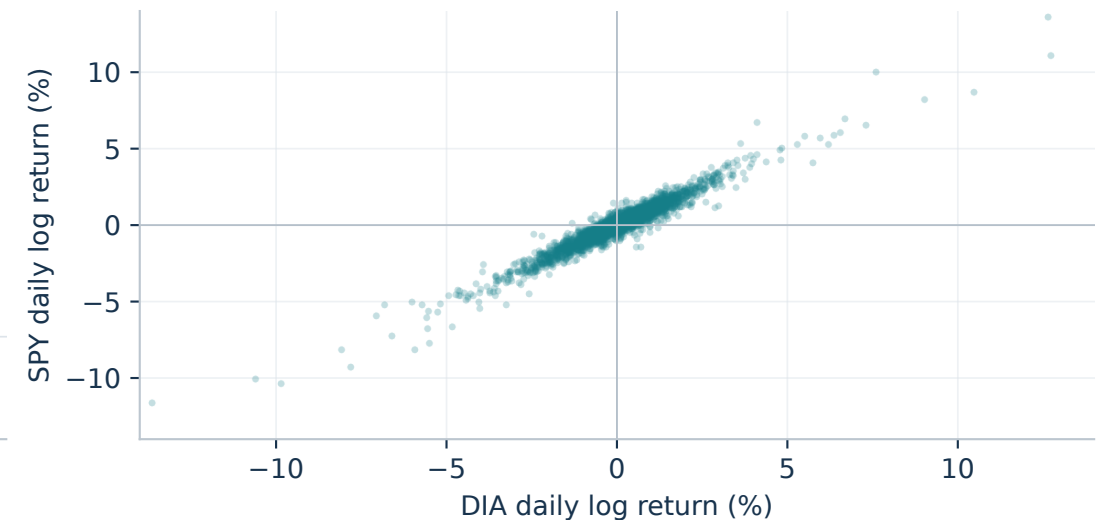
Daily returns: Pearson correlation 0.96
