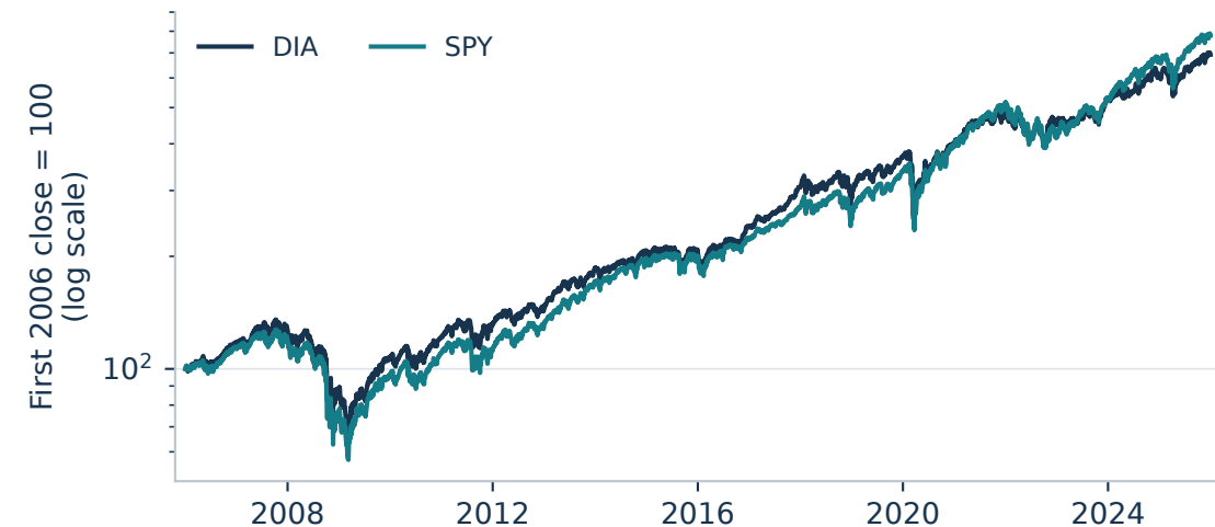
DIA / SPY: adjusted price paths
