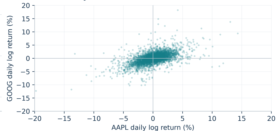
Daily returns: Pearson correlation 0.65
