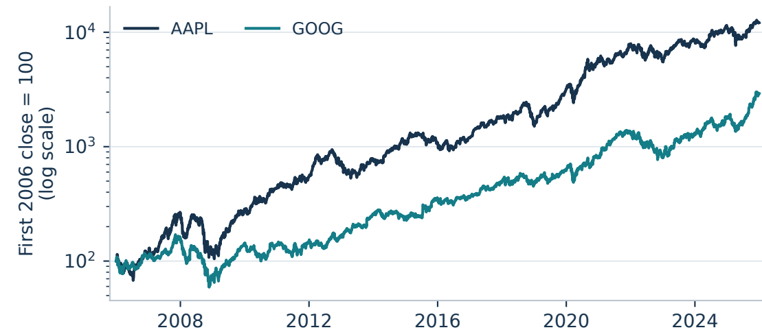
AAPL / GOOG: adjusted price paths
