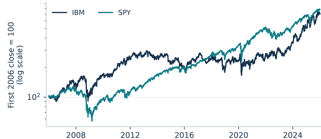
IBM / SPY: adjusted price paths
