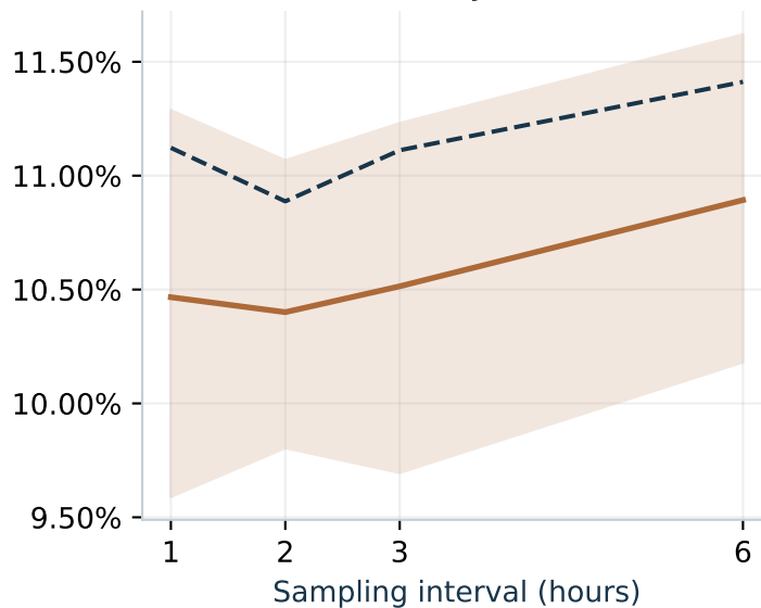
USD/JPY
