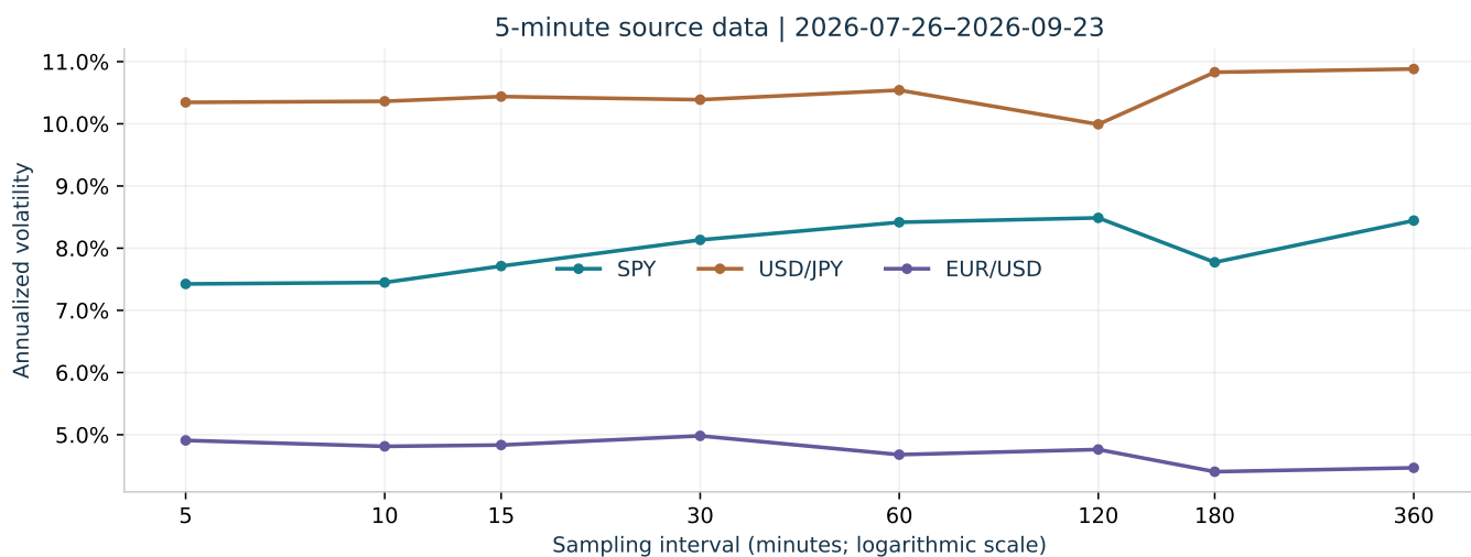
Figure 9. Signatures from the longer five-minute source history, at 5, 10, 15, 30, 60, 120, 180 and 360 minutes. The notebook records return counts, rejected paths and first/last usable timestamps at every interval.
