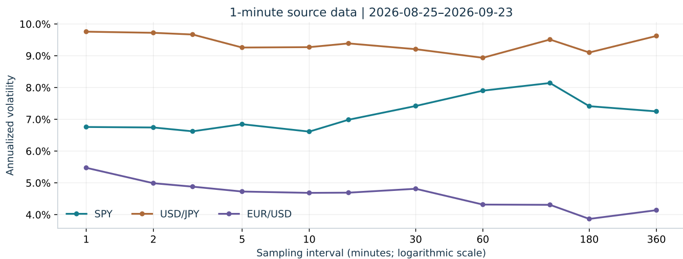
Figure 8. Signatures from one-minute source bars at 1, 2, 3, 5, 10, 15, 30, 60, 120, 180 and 360 minutes. The horizontal axis is logarithmic. Each estimate uses observed, nonoverlapping price paths at its stated interval.
