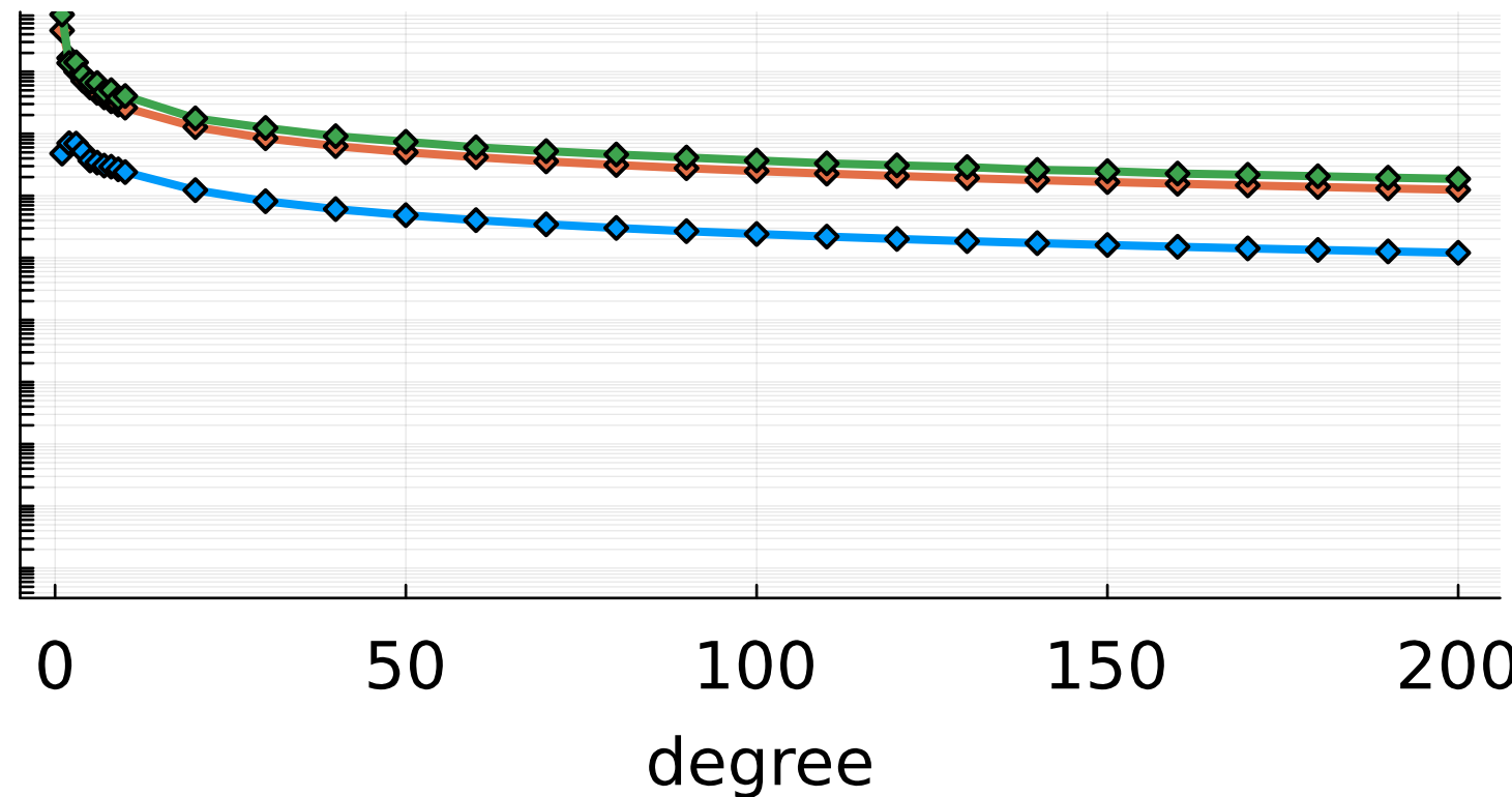
MNIST 256x6
