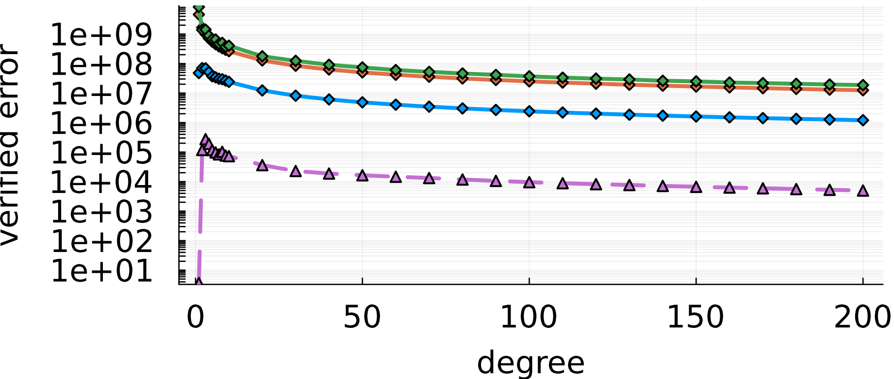
MNIST 256x6
