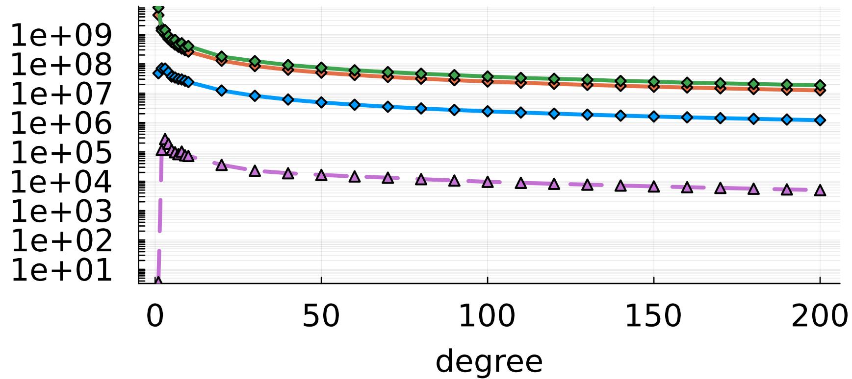
MNIST 256x6
