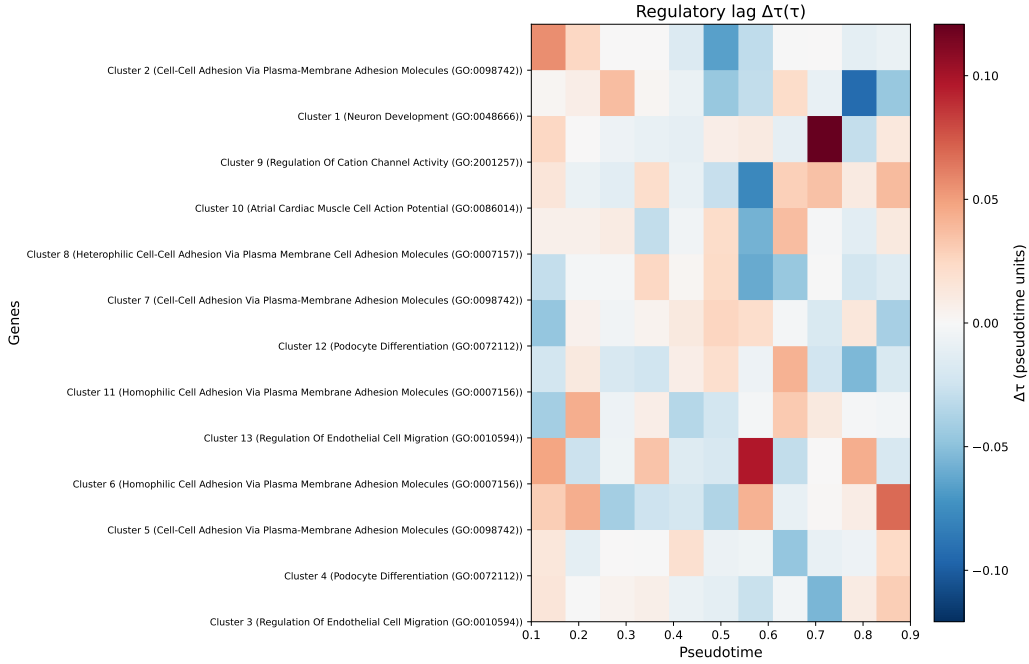
Figure 2: Clustered \Delta\tau heatmap for mouse kidney. Rows are median profiles of 13 clusters (all 50 components were retained after filtering). Red indicates positive \Delta\tau (ATAC leads RNA, priming); blue indicates negative \Delta\tau (RNA leads ATAC, activity-dependent regulation).
