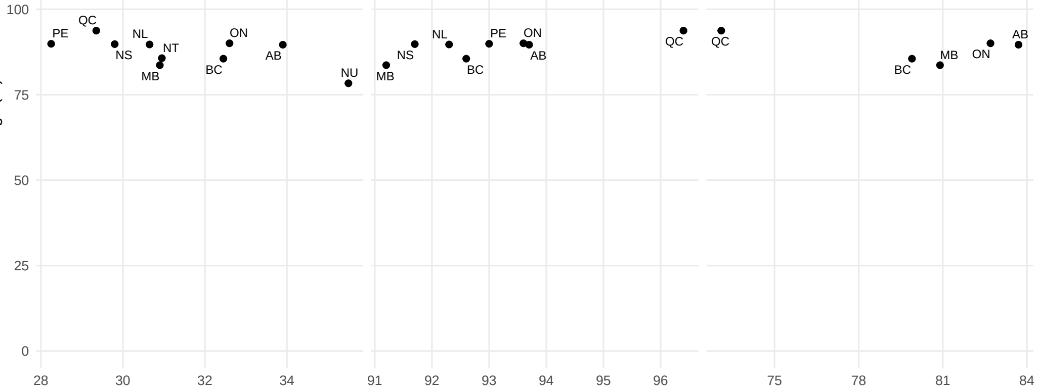
Gini index
