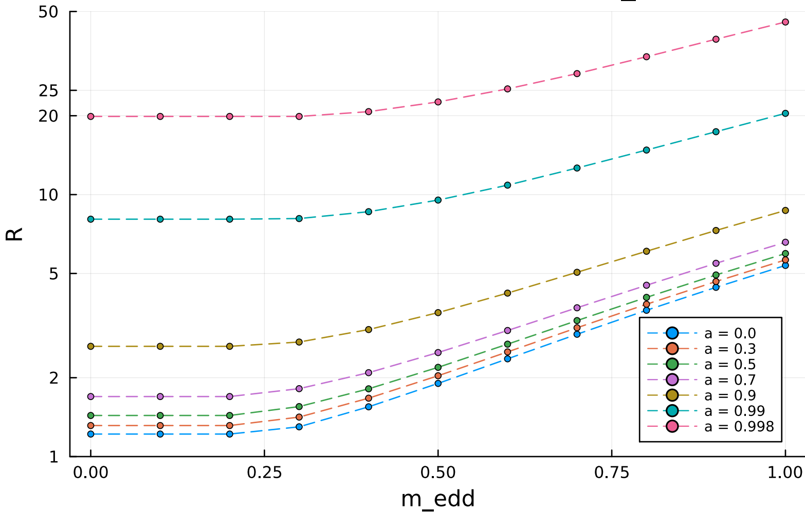
Maximum R as a function of m_{\text{edd}}
